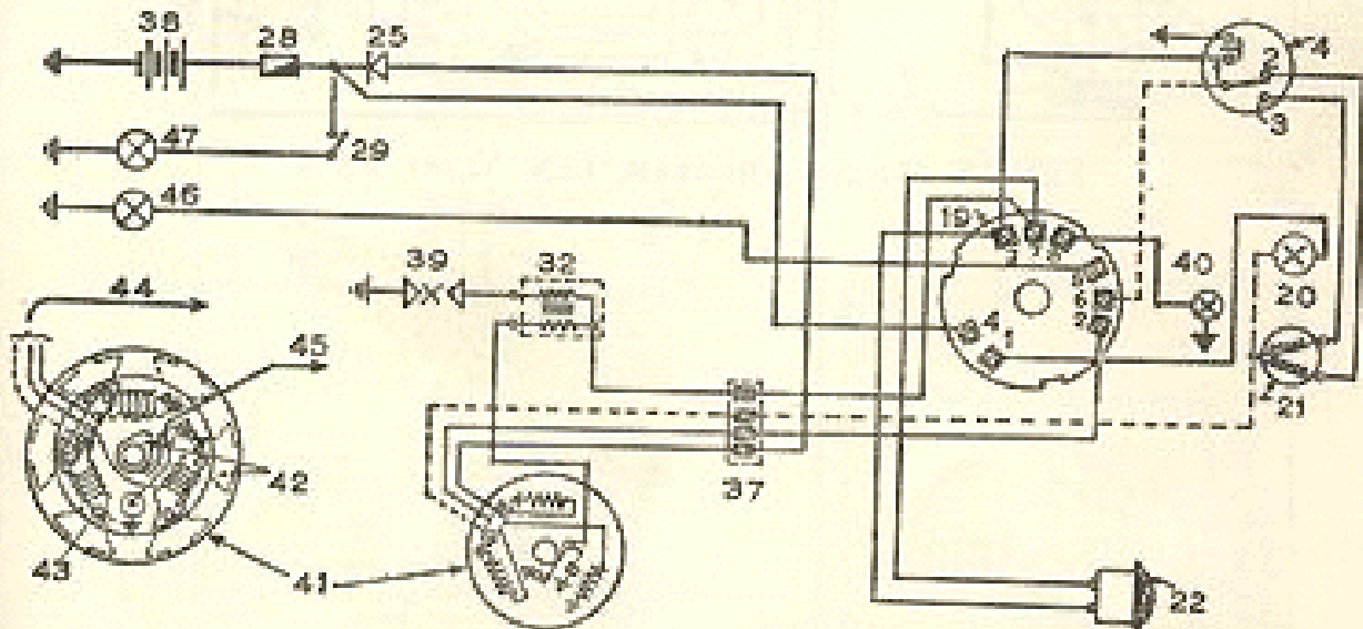
FIG. 34. WIRING DIAGRAM, G.S. VESPA SERIES VS 2
