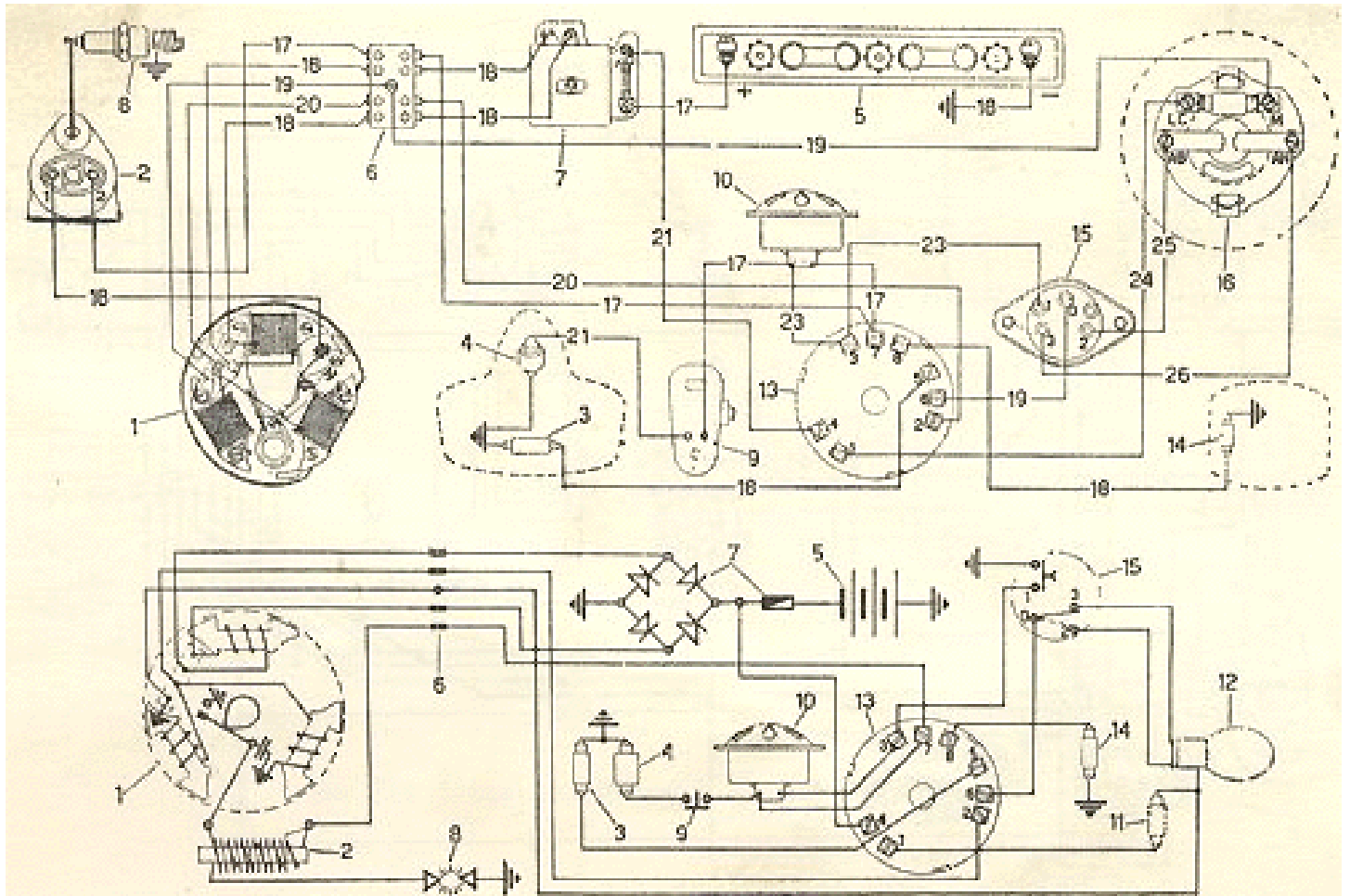
FIG. 36. WIRING DIAGRAM, G.S. VESPA VS5 SERIES
